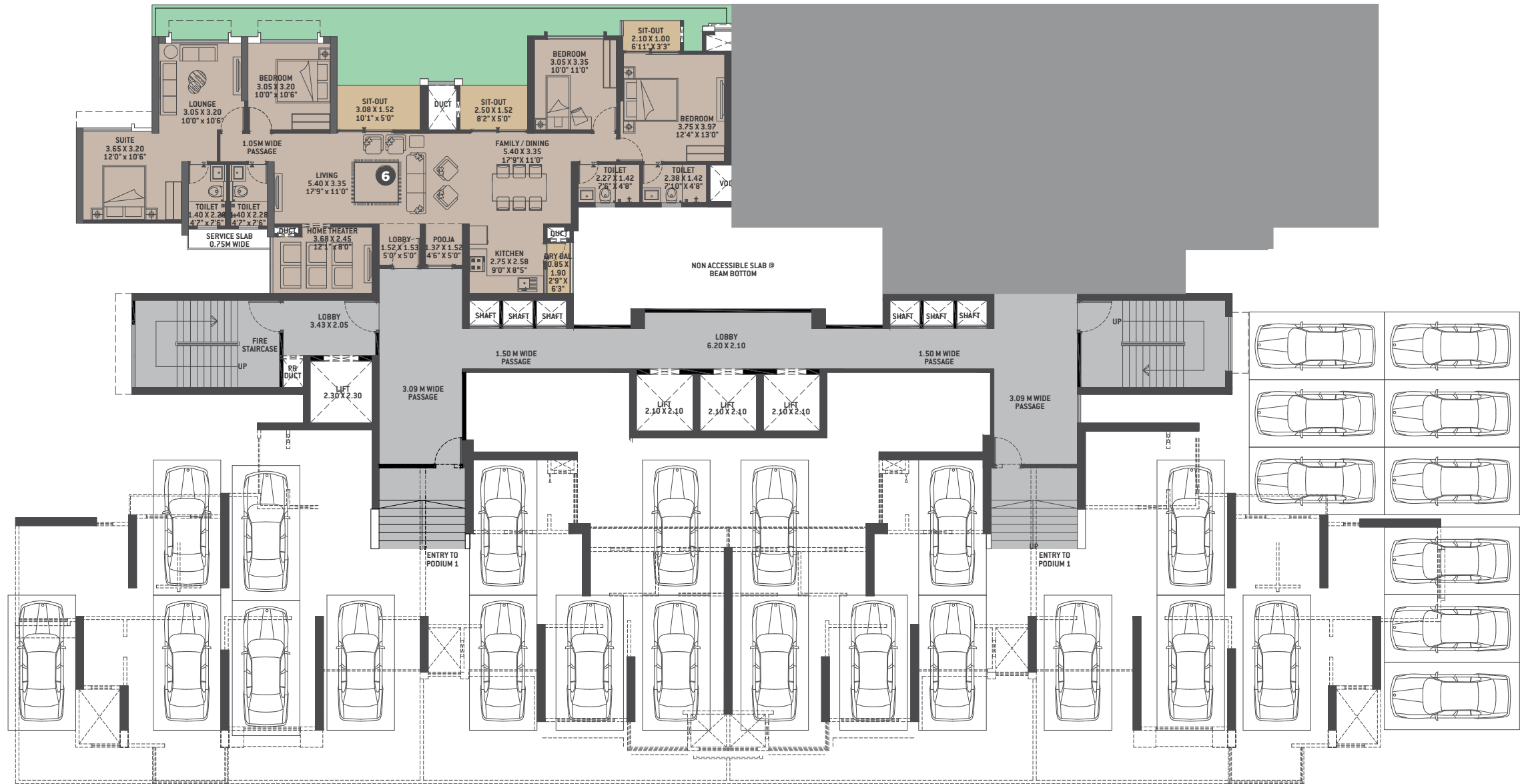
TOWER-3 Podium 1 Floor Plan
