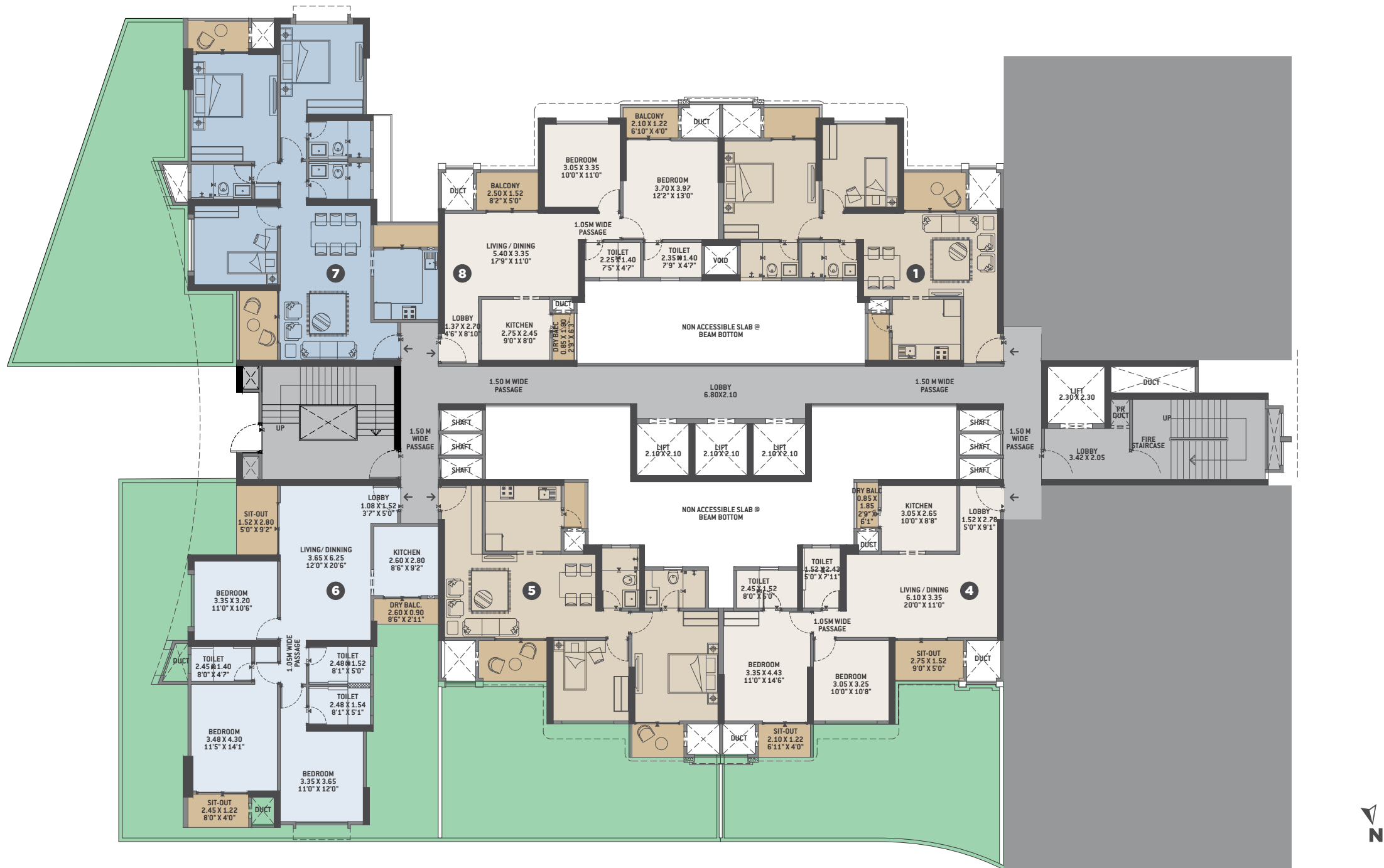
TOWER-1 Podium 3 / First Floor Plan
