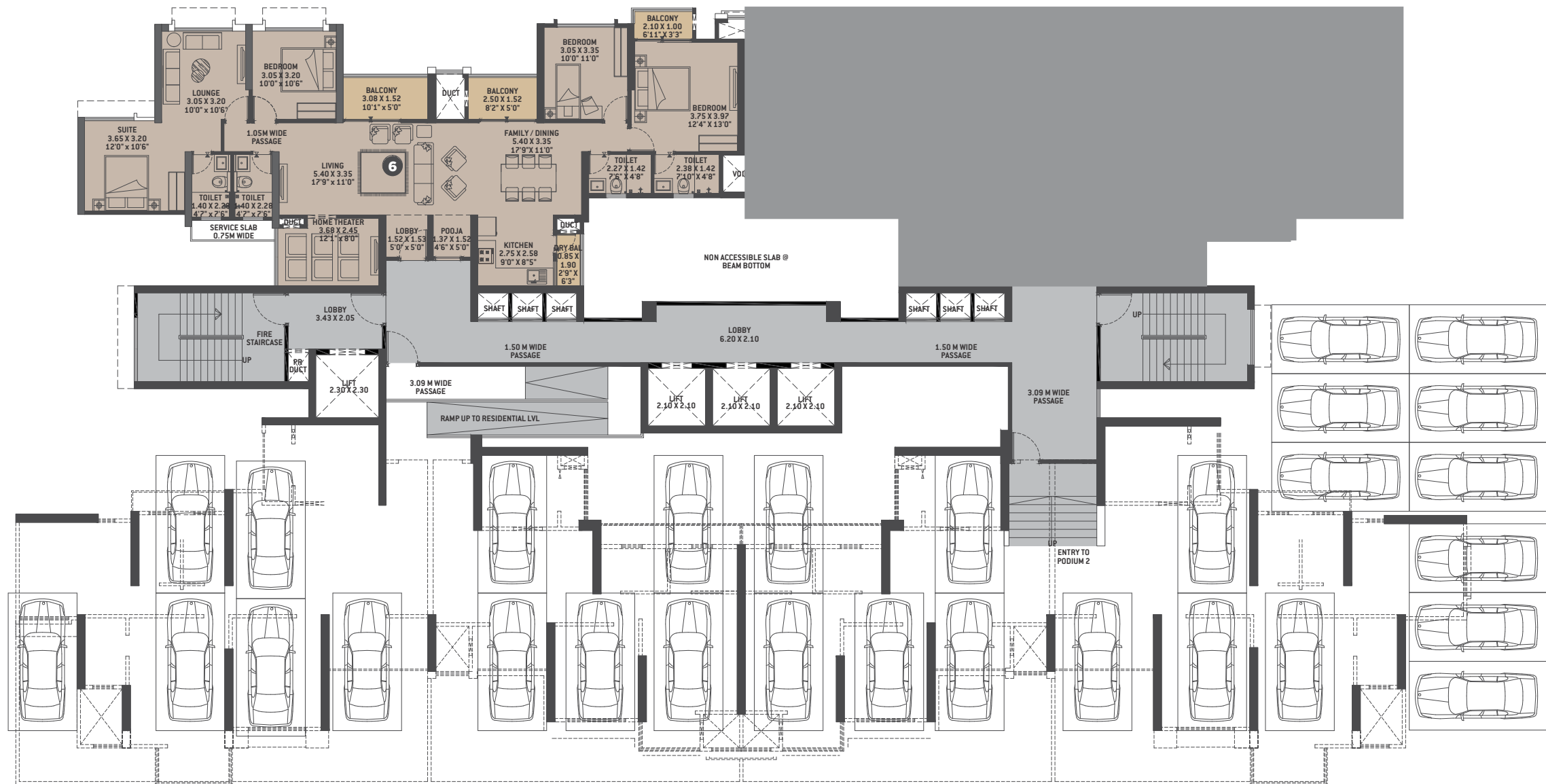
TOWER-3 Podium 2 Floor Plan
