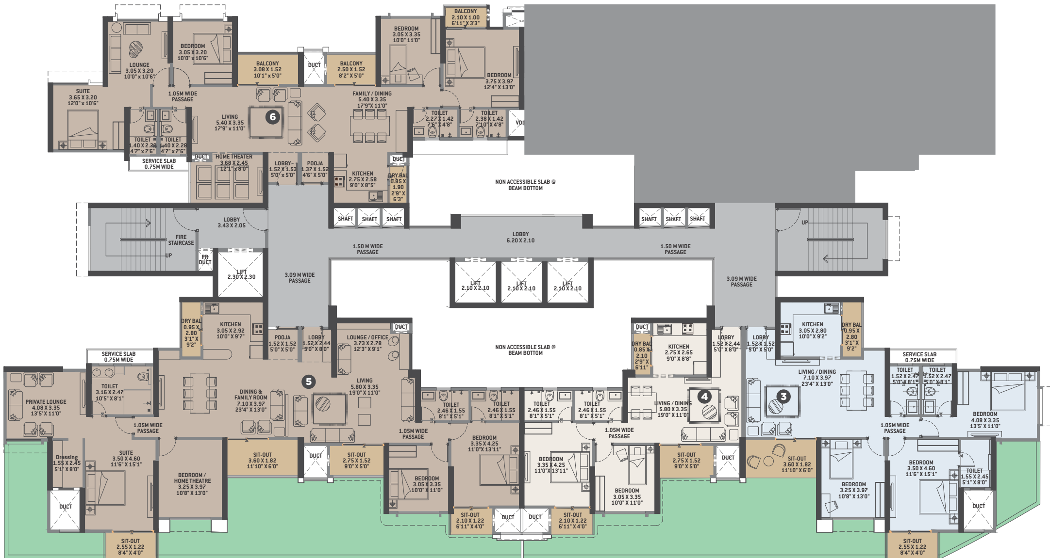
TOWER-3 Podium 3 / First Floor Plan
